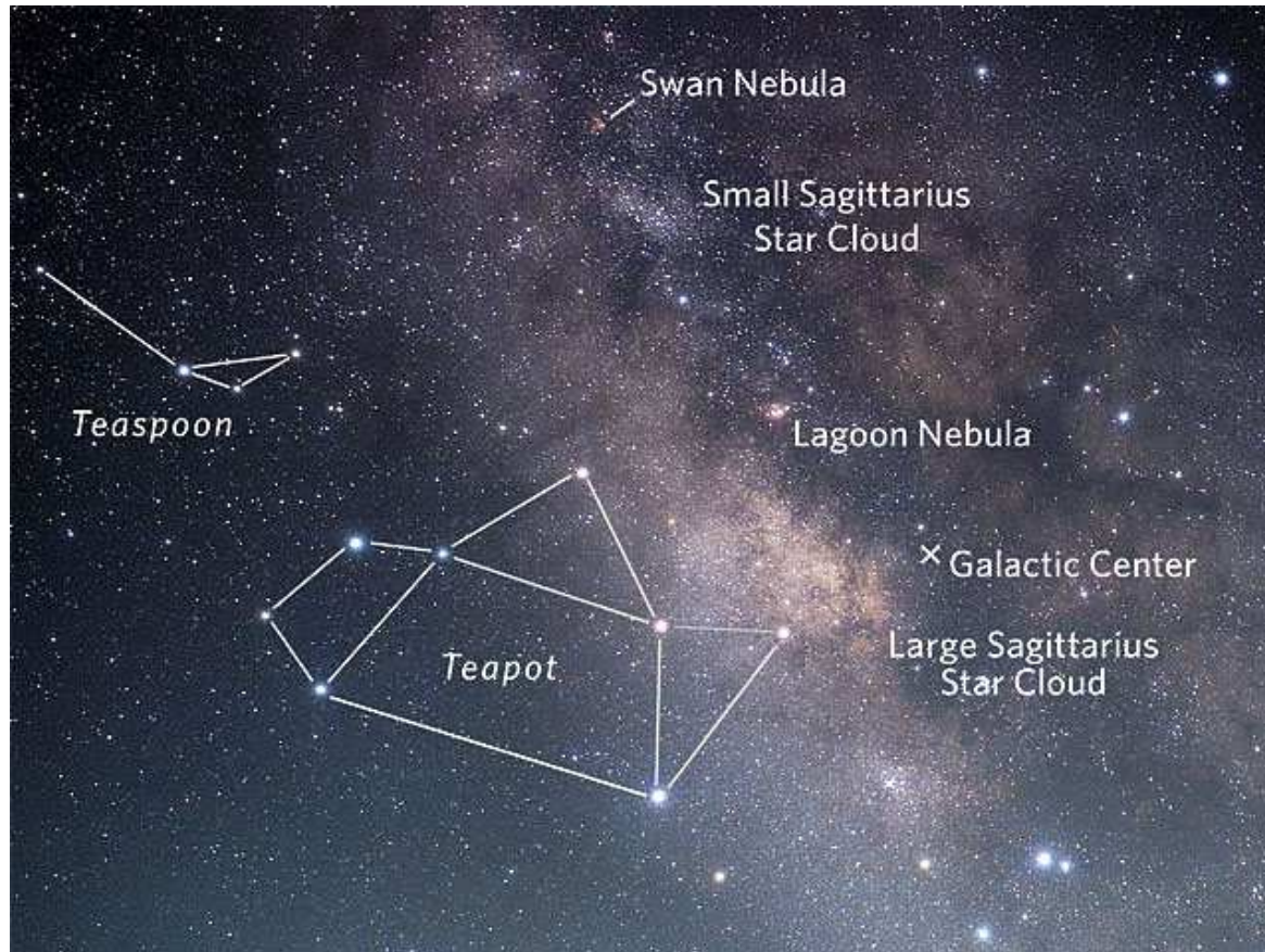
http://www.skyandtelescope.com/wp-content/uploads/Sagittarius-Teapot-Messiers_L.jpg (19.07.2017)
